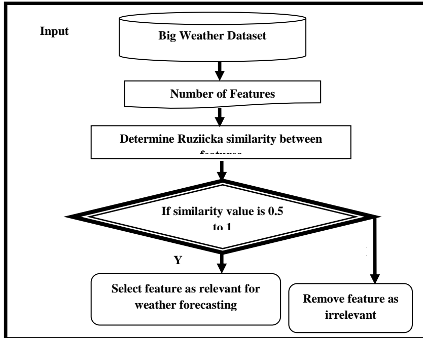
Figure 2 RS-FS algorithm Process for Relevant Feature Selection
