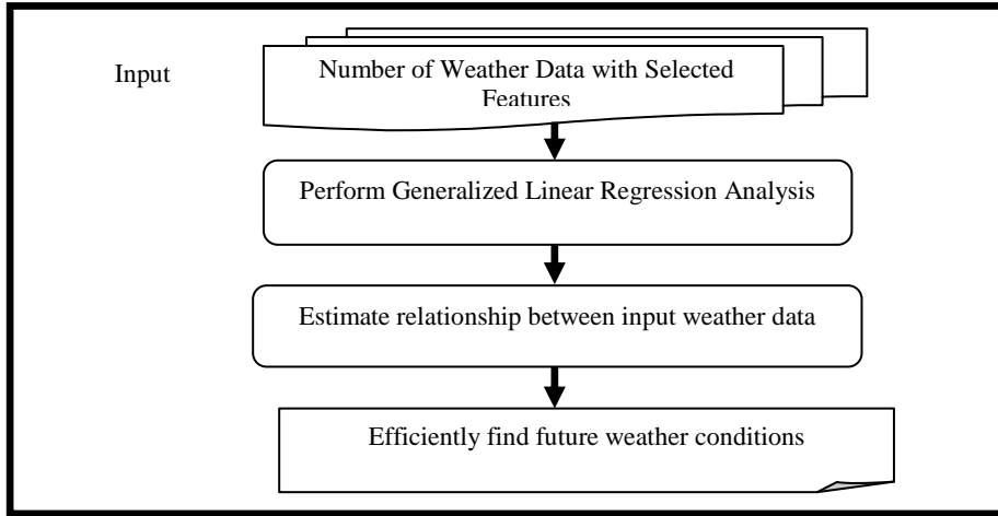
Figure 3 Processes of GLRA-WF algorithm for Weather Forecasting
