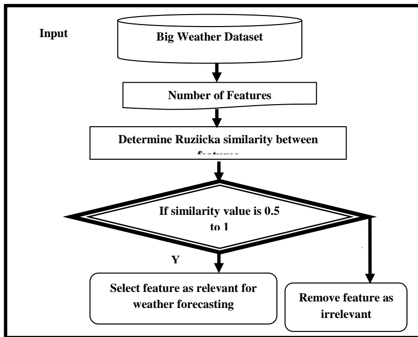
Figure 2 RS-FS algorithm Process for Relevant Feature Selection
