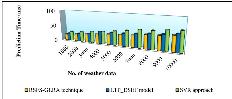
Figure 4 Comparative result of time complexity versus number of weather data
